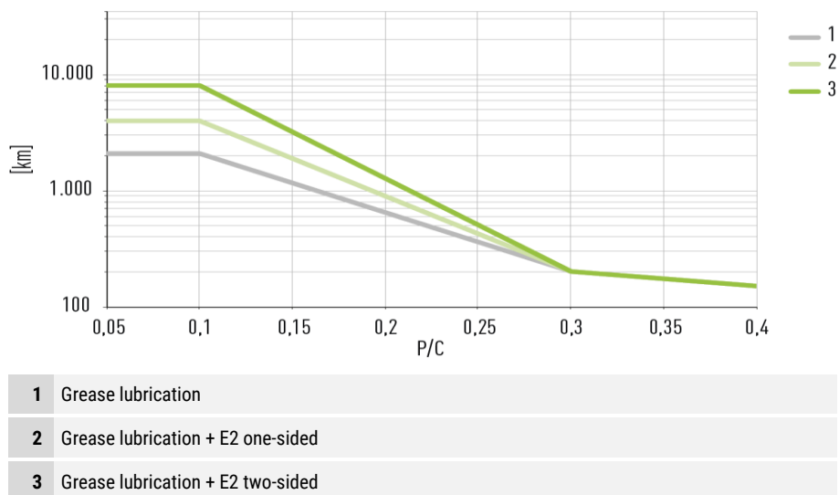
Fig. 8.23: Relubrication intervals with grease lubrication, one-sided and two-sided long-term lubrication unit (E2/EC) for UR and RG.
